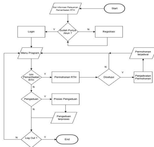
Gambar 2. Flowchart
