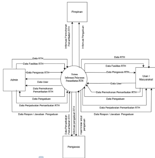
Gambar 3 Data Flow Diagram Level 0
