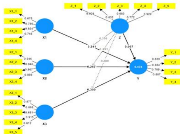
Gambar 1 Output SmartPLS
