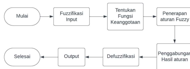
Gambar 2. Flowchart Fuzzy Mamdani
