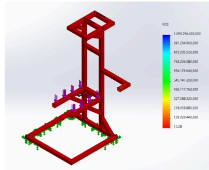
Gambar 9. Hasil Analisis Safety factor
