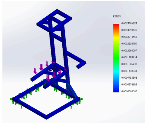
Gambar 8. Hasil Analisis Strain
