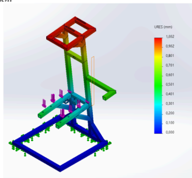
Gambar 7. Hasil Analisis Displacement
