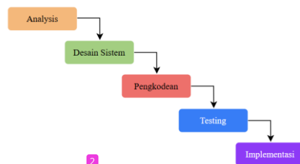
Gambar 1. Metode Waterfall
