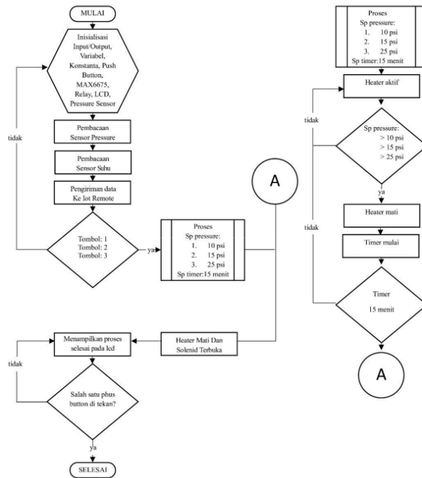
Gambar 2. flowcart sistem
