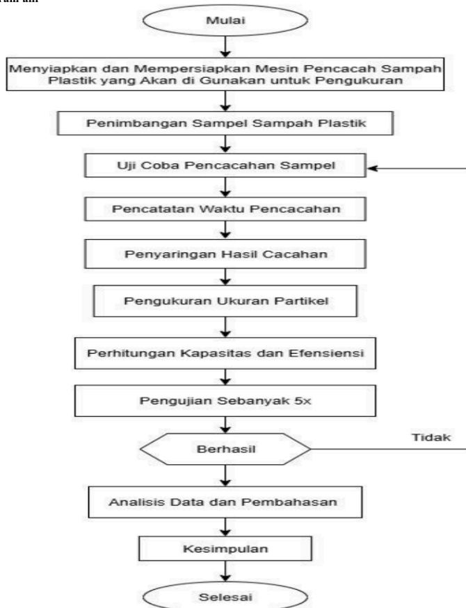
Gambar 1. Diagram Alir
