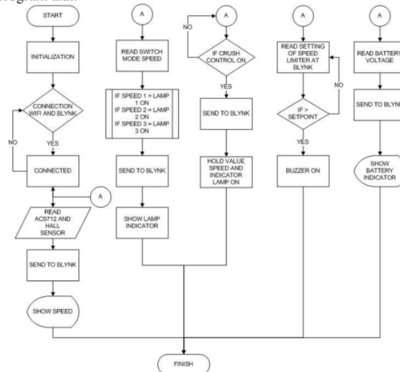
Gambar 3 flowchart program
