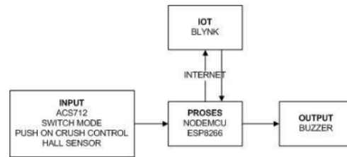
Gambar 2 Diagram Blok
