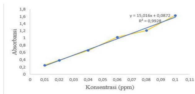
Gambar 2. Kurva standar
