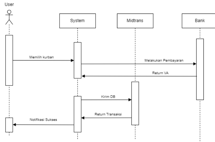
Gambar 8. Sequence Diagram
