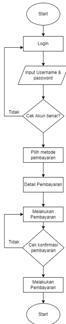
Gambar 2 . Flowchart
