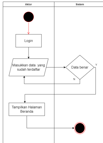
Gambar 5. Activity Diagram Login
