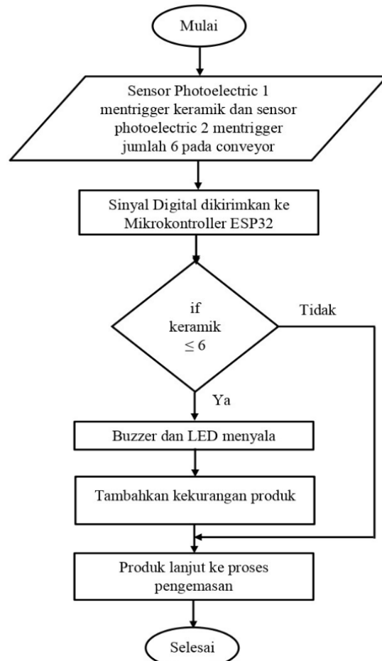
Gambar 2. Flowchart Sistem
