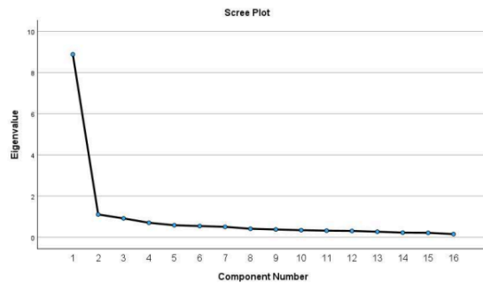
Figure 2. Scree Plot
