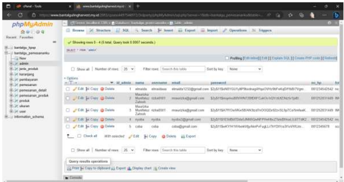
Gambar 20 Halaman DataBase admin
