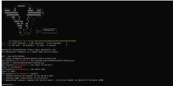
Gambar 3. Tampilan msfconsole
