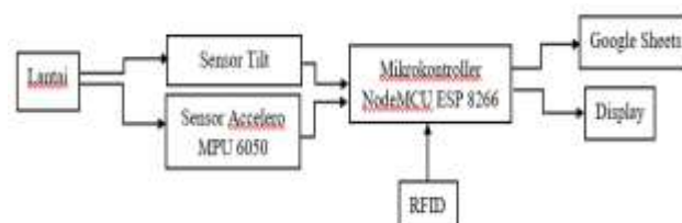
Gambar 1. Diagram Sistem Alat Monitoring Kemiringan Lantai Berbasis Google Sheets
