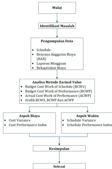
Gambar 1. Flowchart Penelitian
