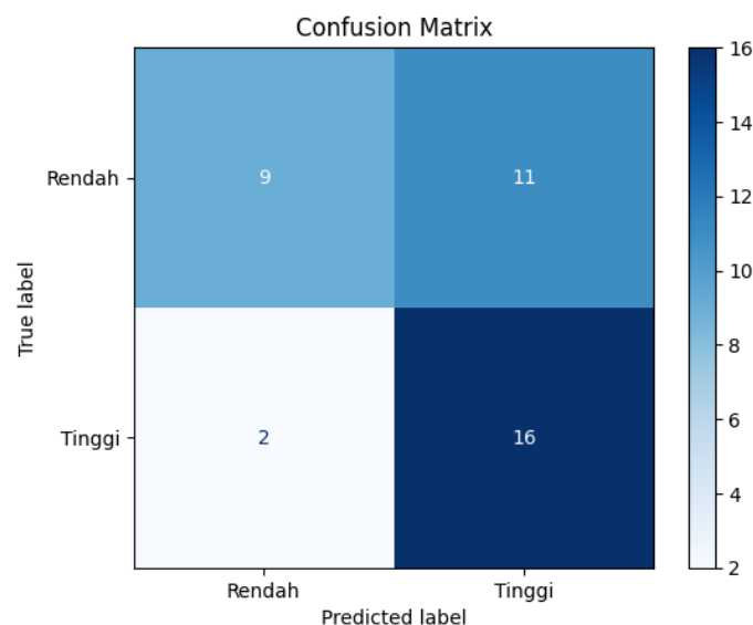
Gambar 2 Confusion Matrix
