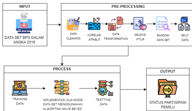
Gambar 1 Alur Penelitian
