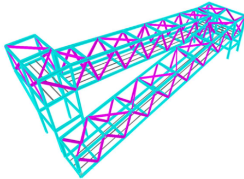
Gambar 4. Model Gangway
