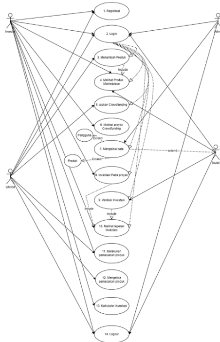
Gambar 1. Usecase Diagram
