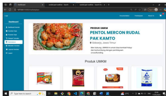
Gambar 19. Halaman Marketplace
