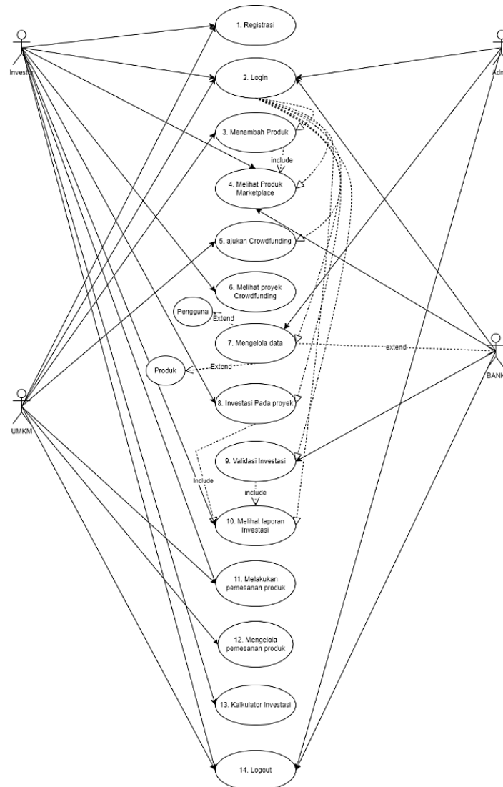
Gambar 1. Usecase Diagram
