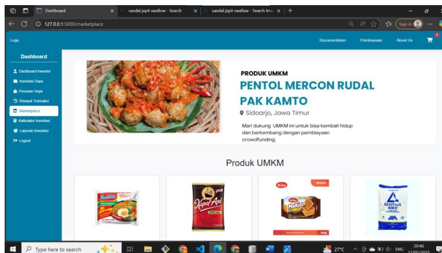
Gambar 19. Halaman Marketplace
