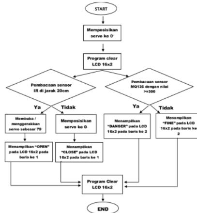
Gambar 3. Flowchart
