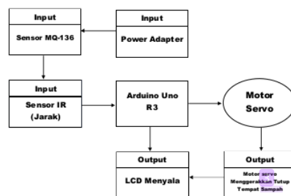
Gambar 1. Diagram Blok
