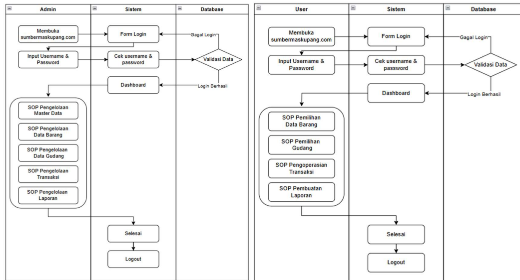
Gambar 3. Flowchart admin dan Flowchart user
