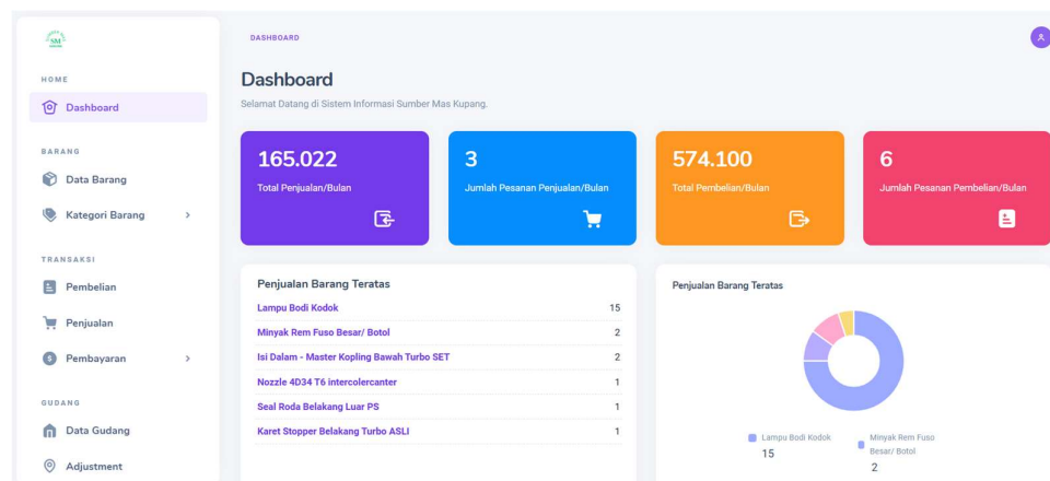
Gambar 15. Tampilan Dashboard
