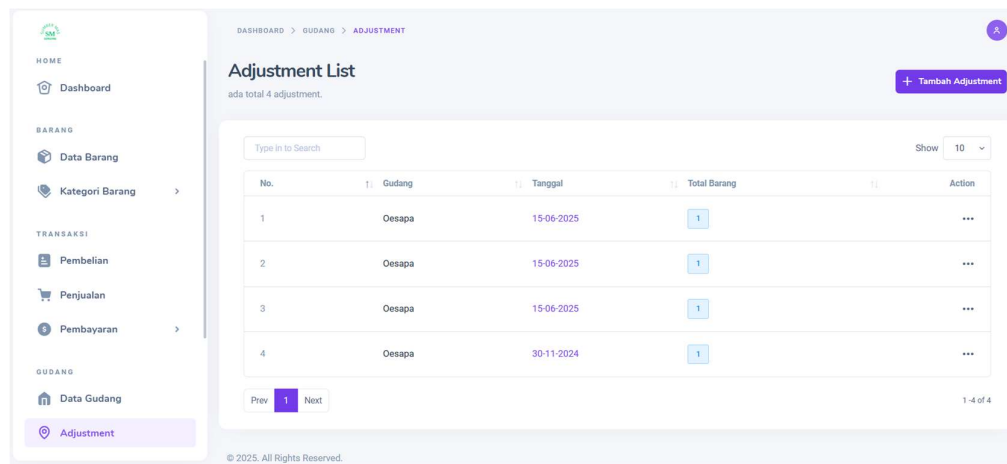
Gambar 22. Tampilan Adjustment
