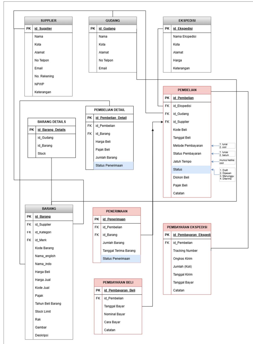
Gambar 4. PDM Pembelian
