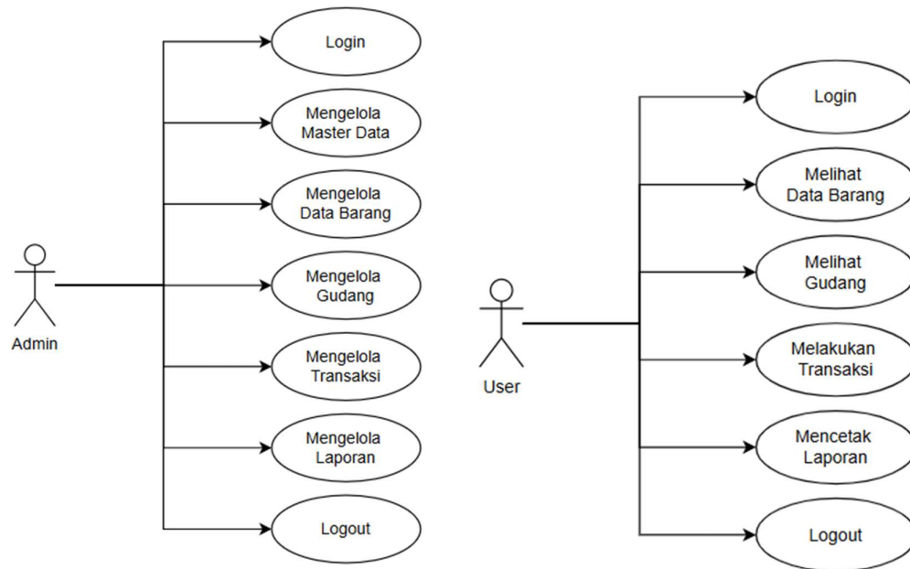
Gambar 2. Use Case Diagram Admin dan Use Case Diagram User
