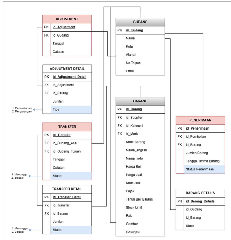
Gambar 6. PDM Persediaan Stok
