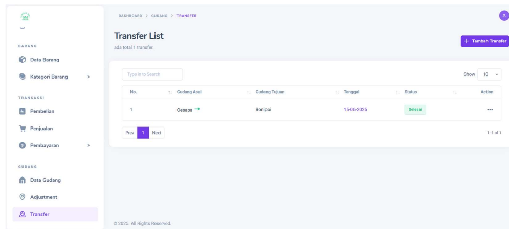
Gambar 23. Tampilan Transfer
