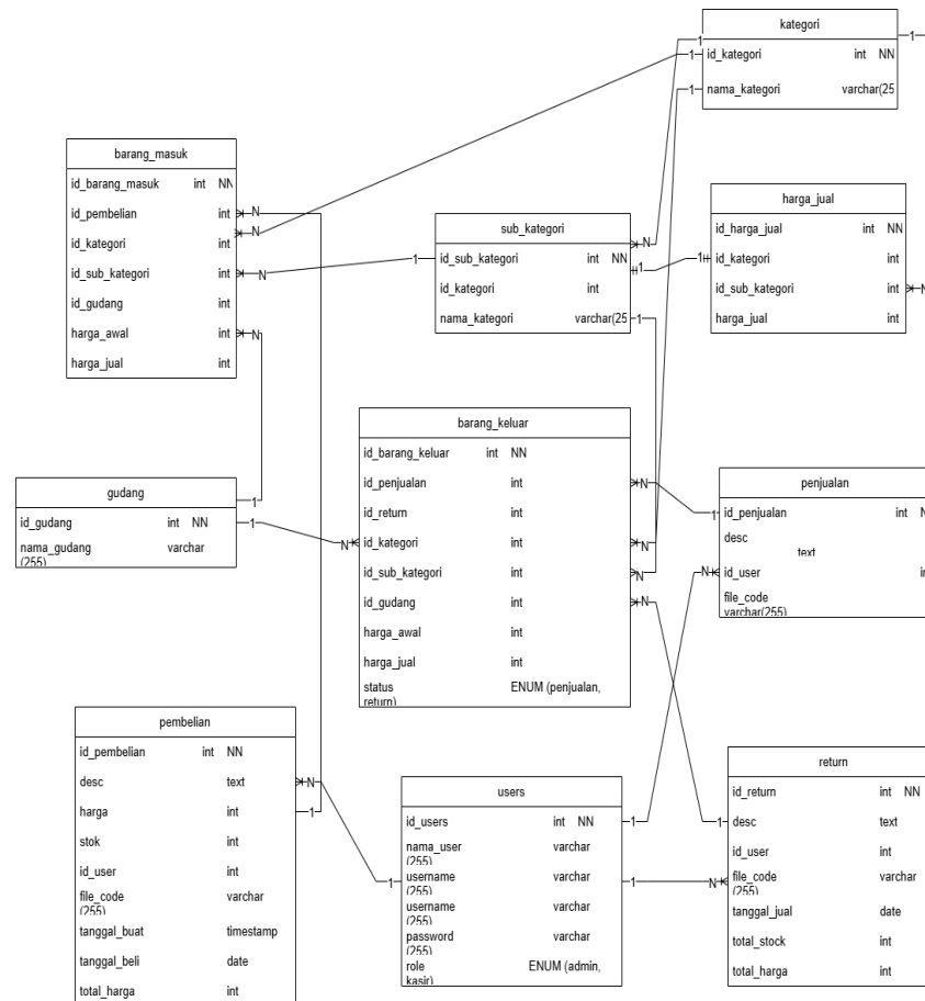
Gambar 4. ERD (Entity Relationship Diagram)
