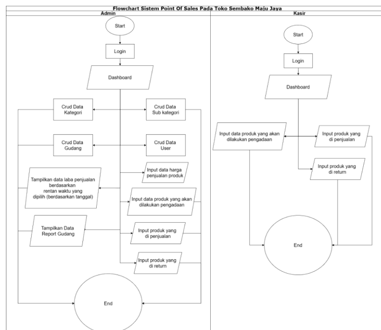
Gambar 1. Flowmap Sistem Usulan
