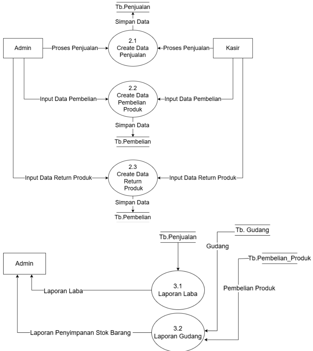
Gambar 3. DFD level 1
