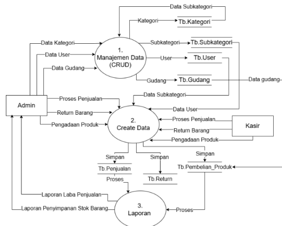
Gambar 2. DFD level 0
