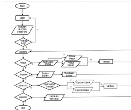
Gambar 1. Flowchart Admin
