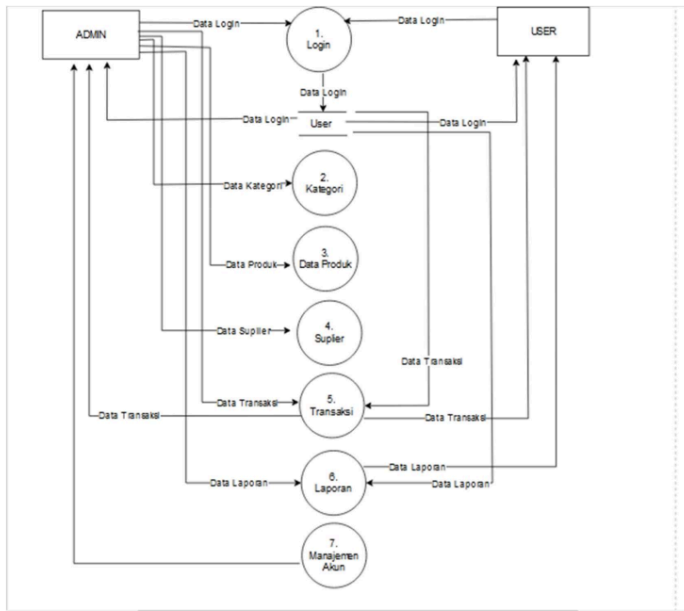
Gambar 4. DFD level 1
