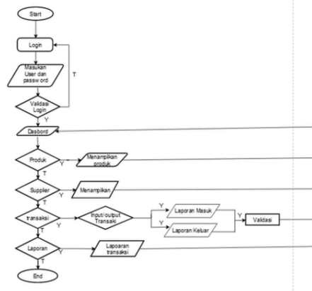
Gambar 2. Flowchart User
