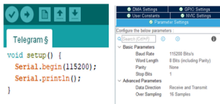
Gambar 8. Kode Program
