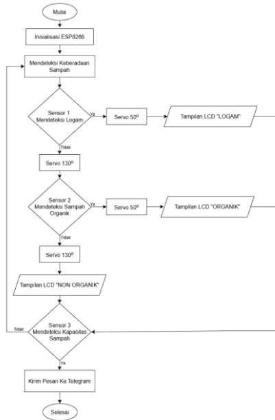
Gambar 3. Flowchart
