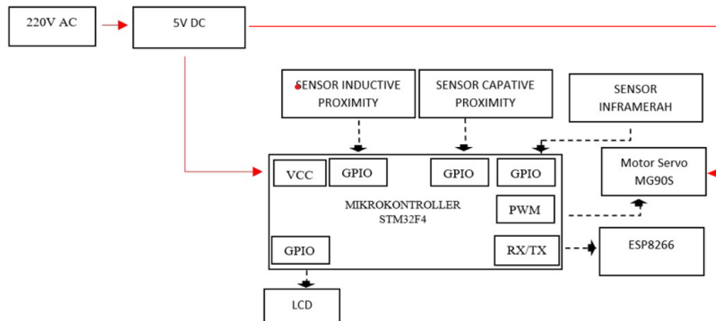
Gambar 2. Diagram Blok
