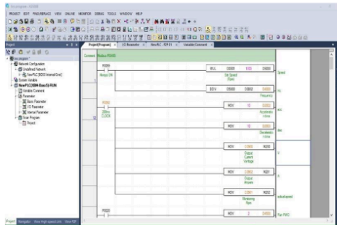
Gambar 3. Ladder Program PLC
