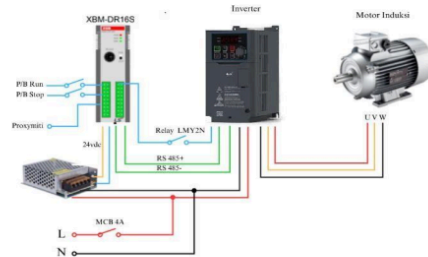
Gambar 1. Skema wiring diagram rangkaian Modbus Rtu Rs-485
