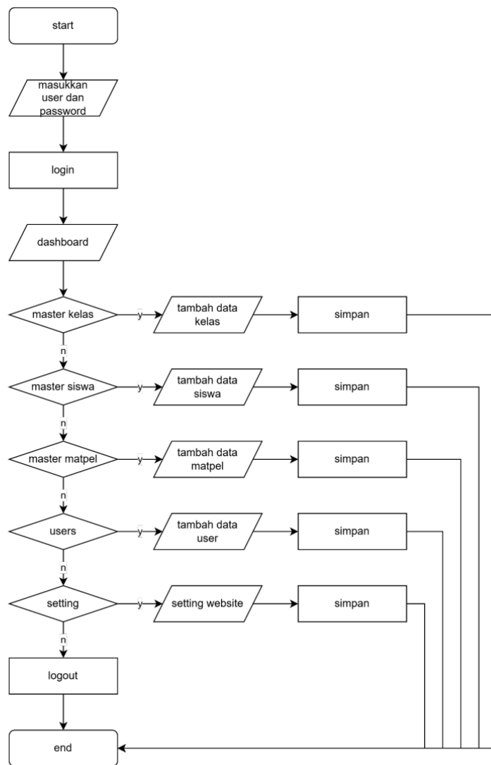
Gambar 1. Flowchart Admin
