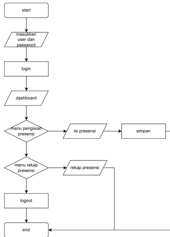
Gambar 2. Flowchart Guru
