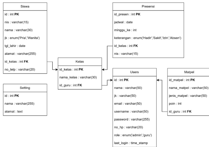
Gambar 5. Class Diagram
