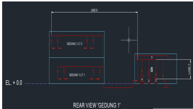
Gambar 2 Instalasi Line Pipa Hydrant Indoor
