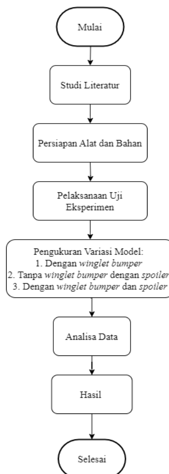
Gambar 3. Flowchart
