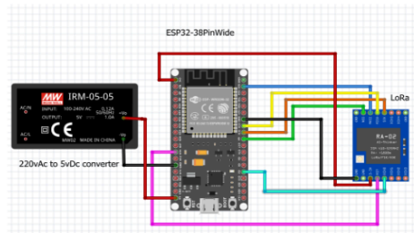
Gambar 5. Rangkaian Receiver
