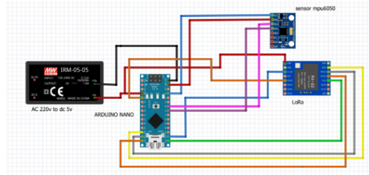
Gambar 4. rangkaian node transmitter
