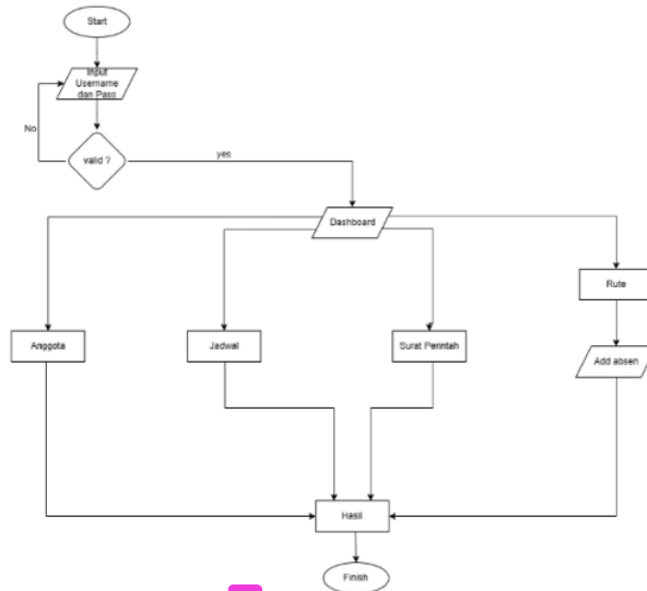
14 Gambar 3. Flowchart User
