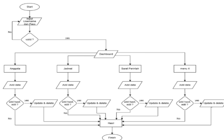
Gambar 2. Flowchart Admin
