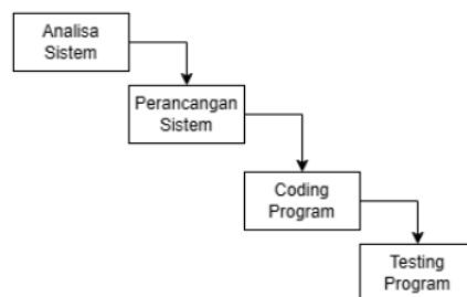
Gambar 1. Metode Waterfall
