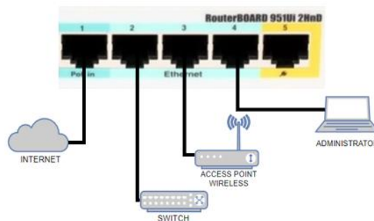
Gambar 5. Detail Persebaran Port Router
