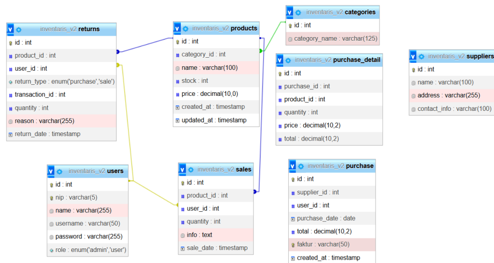
Gambar 4. Relasi basis data
