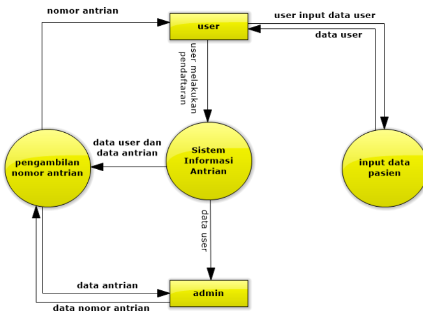
Gambar 4, DFD Level 0
