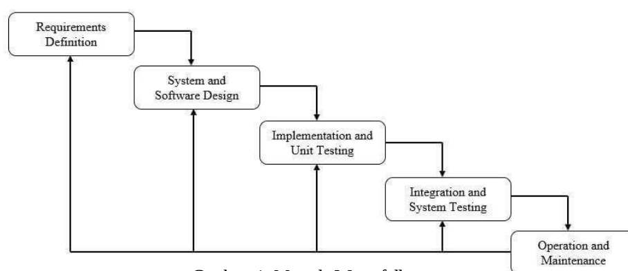
Gambar 1. Metode Waterfall
