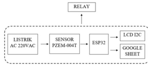
Gambar 2. Blok Diagram
