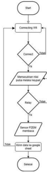
Gambar 3. Flowchart
