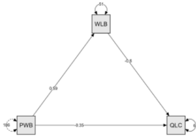
Gambar 3. Path Plot
