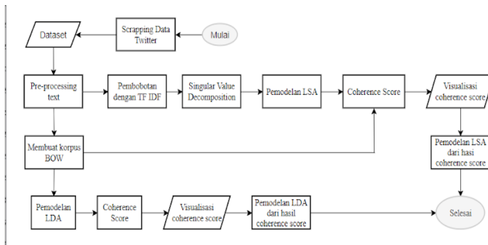
Gambar 1. Flowchart Penelitian
