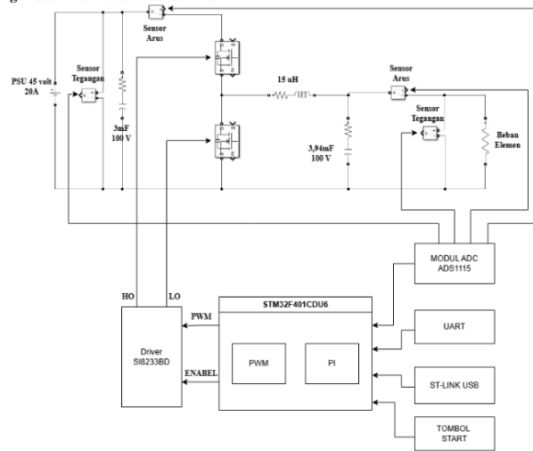
Gambar 5. Blok diagram Konverter Buck Sinkron
