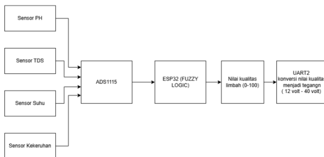
Gambar 8. Diagram Sistem Modul Kontrol Sensor Limbah
