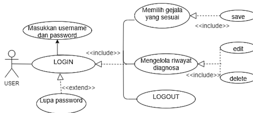
Gambar 3. Usecase diagram user
