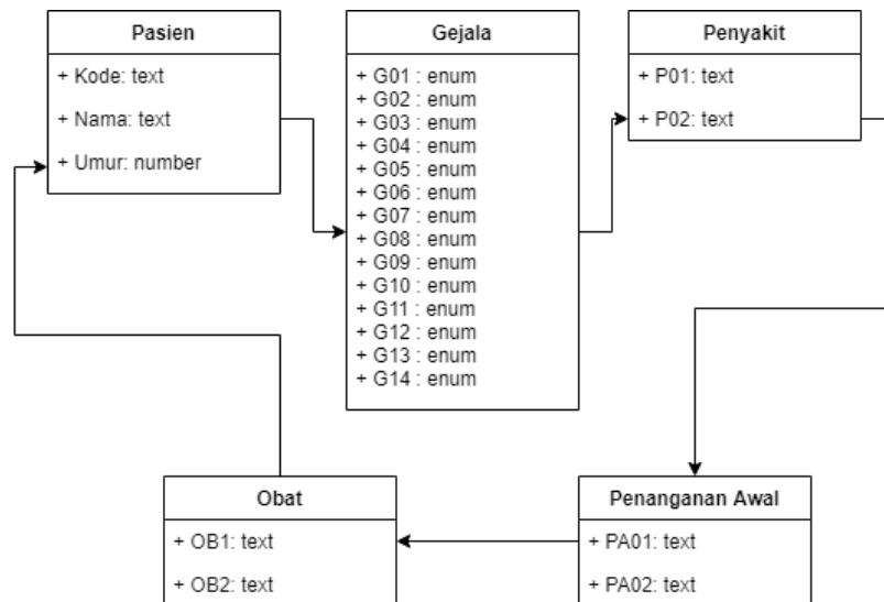
Gambar 6. Entitas rancangan basis data
