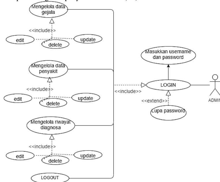
Gambar 2. Usecase diagram admin
