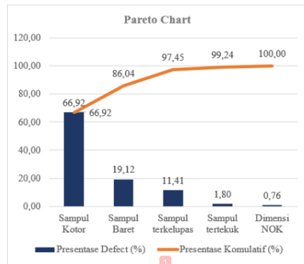
Gambar 3. Diagram Pareto
