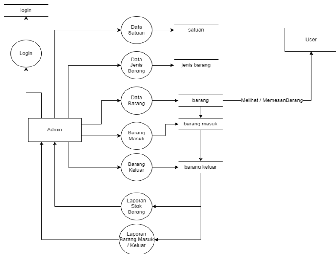
Gambar 3. DFD Level 1
