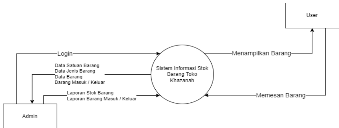
Gambar 2. DFD Level 0
