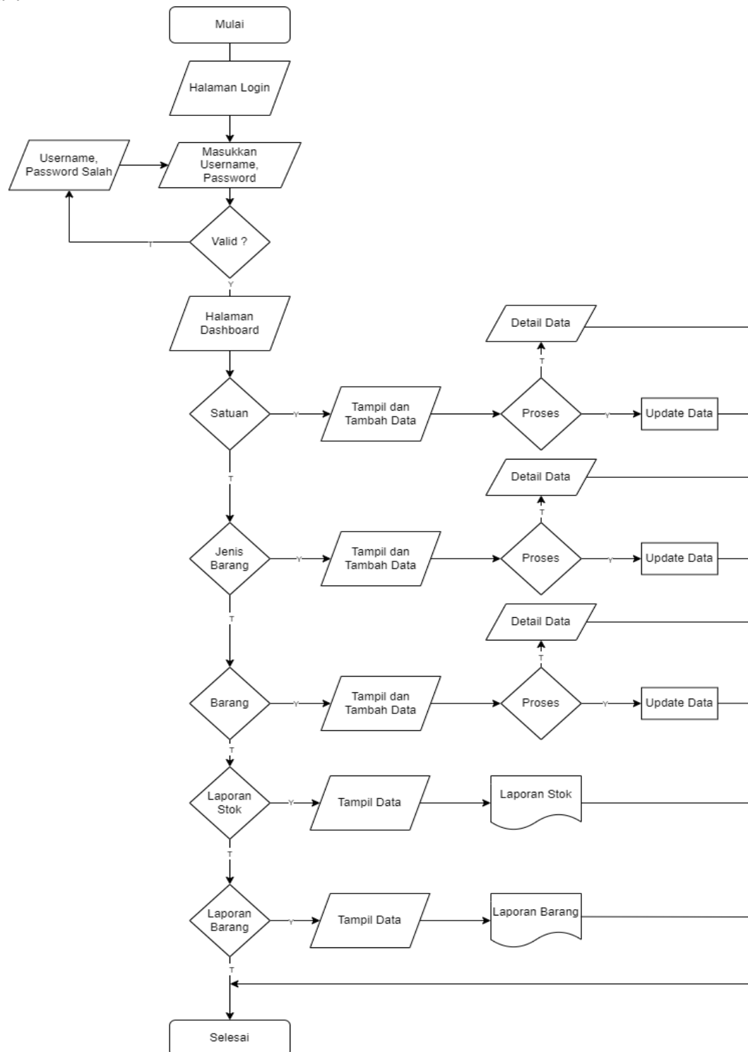
Gambar 1. Flowchart
