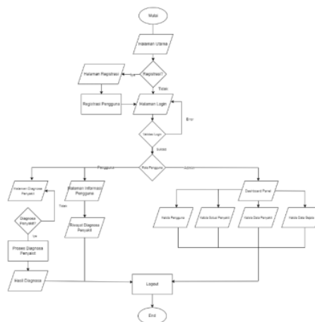
Gambar 2. Flowchart Sistem Pakar
