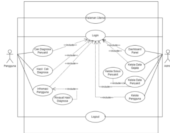
15 Gambar 3. Use Case Diagram Sistem Pakar
