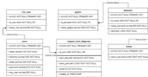
Gambar 4. Class Diagram Sistem Pakar
