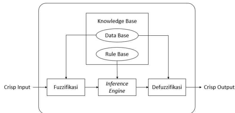
Gambar 1. Fuzzy Logic [29]
