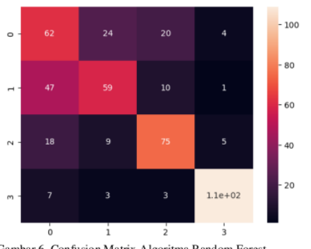
Gambar 6. Confusion Matrix Algoritma Random Forest
