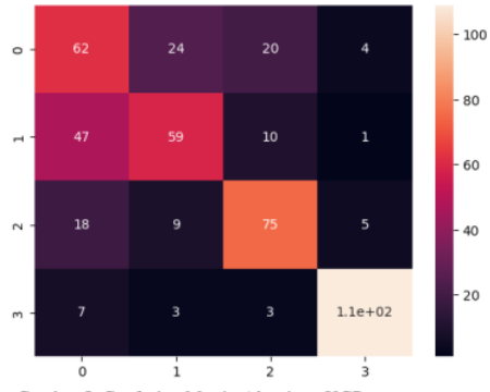
Gambar 5. Confusion Matrix Algoritma XGBoost
