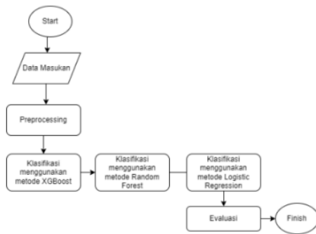
Gambar 1. Alur Penelitian
