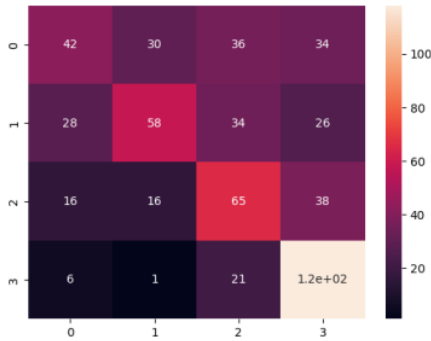
Gambar 7. Confusion Matrix Algoritma Logistic Regression
