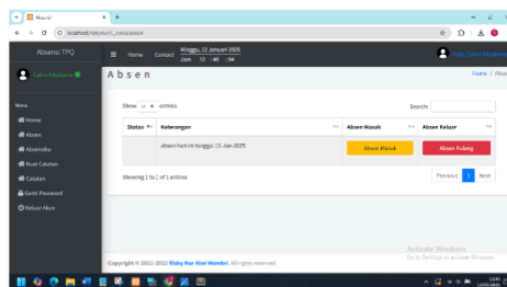
Gambar 15. Pengisian Absen
