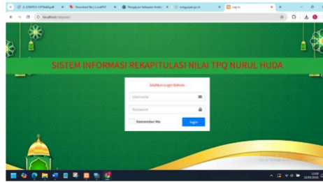
Gambar 4. Halaman Admin
