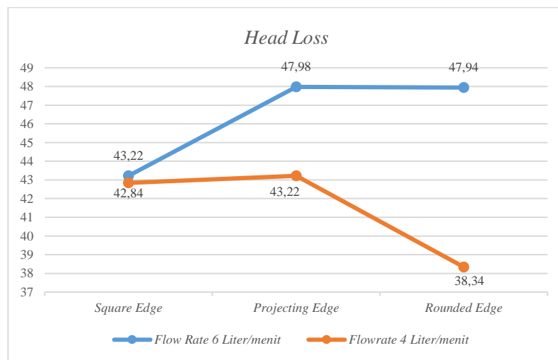
Gambar 2. Grafik Head Loss
