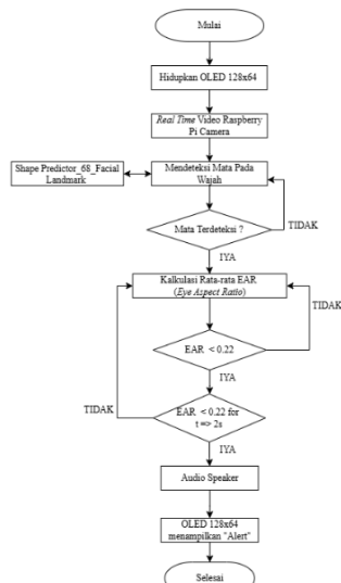
Gambar 3. Diagram Alir
