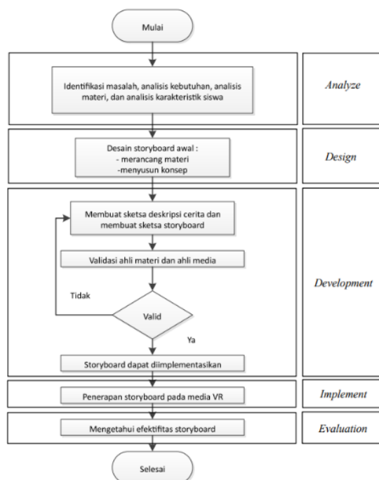
Gambar 1. Prosedur pengembangan Storyboard ADDIE
