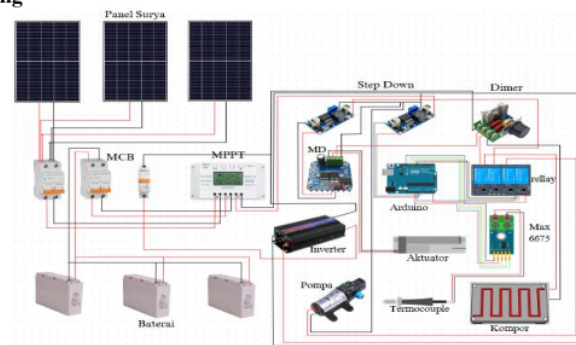
Gambar 3. Wiring Diagram Sistem
